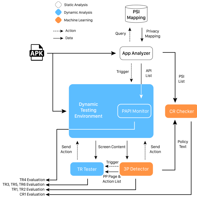
Fig. 1: Analysis Workflow.
